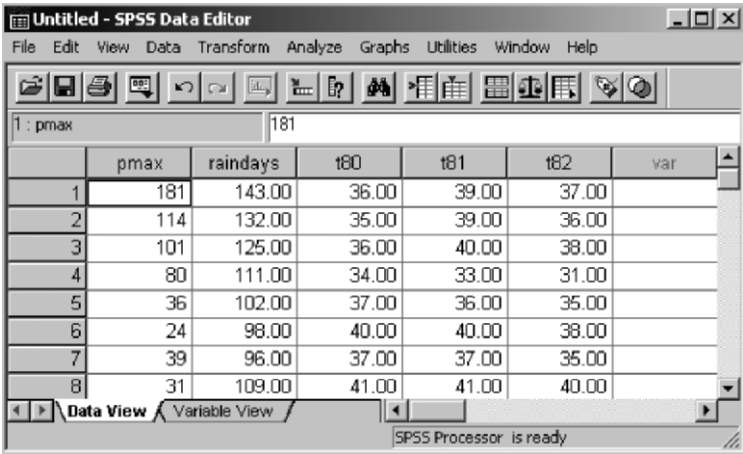
Figure 2.2. Data View spreadsheet of SPSS for the meteorological data.
