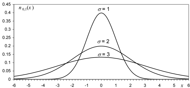
Figure B.9. Normal density function with zero mean for three different values of \sigma .
