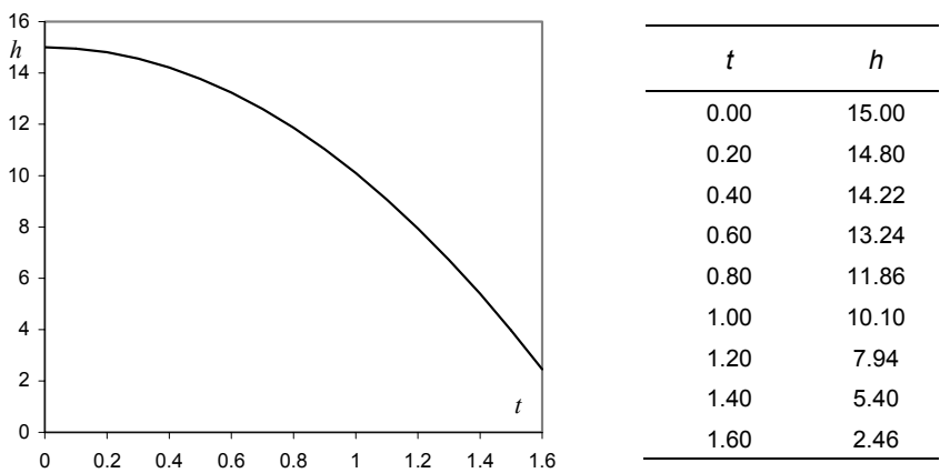
Figure 1.1. Body in free-fall, with height in meters and time in seconds, assuming g = 9.8 \text{ m/s}^2 . The h column is an example of deterministic data.
