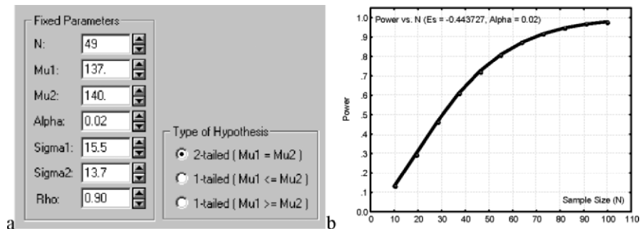
Figure 5.7. Determining the power for a two-paired samples t test, with STATISTICA: a) Specification window, b) Power curve dependent on n .
