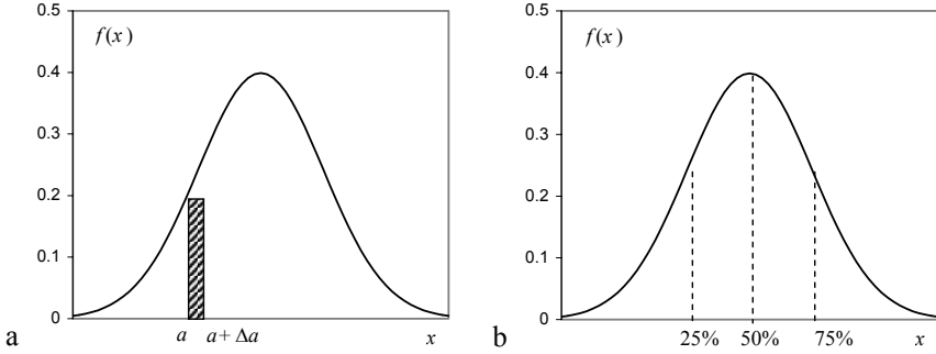
Figure A.3. a) A pdf example; the shaded area in [a, a + \Delta a] is an infinitesimal probability mass. b) Interesting points of a pdf: lower quartile (25% of the total area); median (50% of the total area); upper quartile (75% of the total area).
