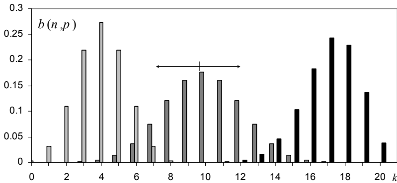
Figure B.5. Binomial probability functions: B_{8, 0.5} (light grey); B_{20, 0.5} (dark grey); B_{20, 0.85} (black). The double arrow indicates the \mu \pm \sigma interval for B_{20, 0.5} .
