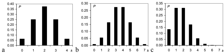
Figure 5.6. Binomial distributions for the sign tests in Example 5.18: a) TW-CI pair, under H_0 ; b) MC-MA pair, under H_0 ; c) MC-MA pair for the alternative hypothesis H_1 : P(\text{MC} < \text{MA}) = \frac{1}{4} .
