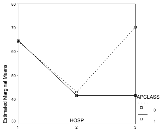
Figure 4.20. Plot of estimated marginal means for Example 4.20. SPSS and STATISTICA provide the possibility of testing contrasts in multi-way ANOVA analysis. With STATISTICA, the user fills in at will the contrast coefficients in a specific window (e.g. click Specify contrasts for LS means in the Planned comps tab of the ANOVA command, with HOSP*APCLASS interaction effect selected). SPSS follows the approach of computing an exhaustive set of contrasts.
