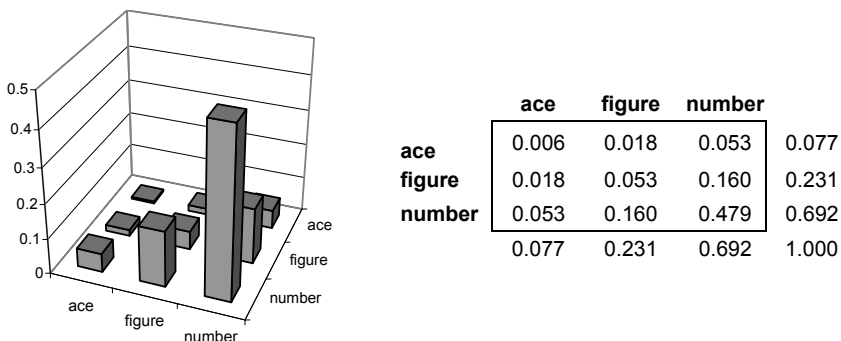
Figure A.1. Sample space and probabilities corresponding to the compound card drawing experiment.
