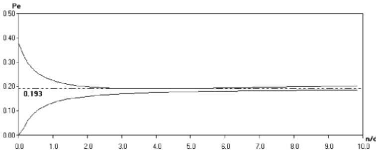
Figure 6.15. Two-class linear discriminant E[\hat{Pe}_d(n)] and E[\hat{Pe}_t(n)] curves, for d = 7 and \delta^2 = 3 , below and above the dotted line, respectively. The dotted line represents the Bayes error (0.193).
