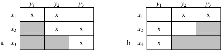
Figure 2.27. Examples of contingency table formats for: a) G = 1 ( N_{ij}^- cells are shaded gray); b) G = -1 ( N_{ij}^+ cells are shaded gray).
