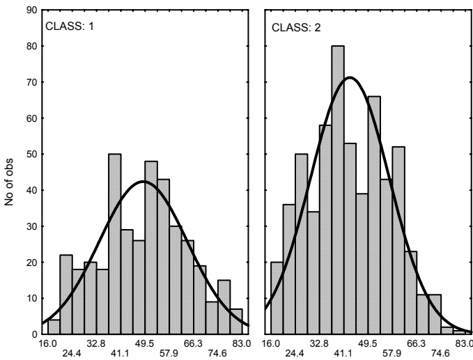
Figure 3.6. Histograms obtained with STATISTICA of the variable ASTV (percentage of abnormal beat-to-beat variability), for the first two classes of the cardiocotographic data, with superimposed normal fit.
