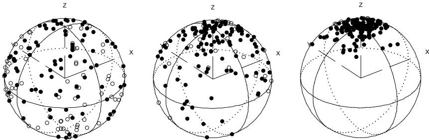
Figure 10.5. Spherical plots of 150-point-samples with von Mises-Fisher distribution around [0 \ 0 \ 1]' , and \kappa = 0.001, 2, 10 , from left to right, respectively.
