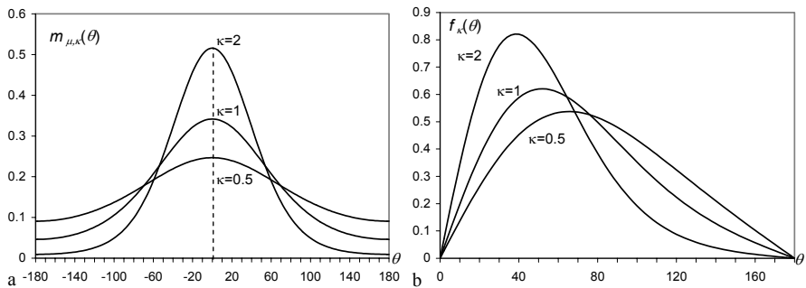
Example B. 17. a) Density function of the circular von Mises distribution for \mu = 0 and several values of \kappa ; b) Density function of the co-latitude of the spherical von Mises distribution for several values of \kappa .
