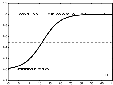
Figure 7.24. Logistic response for the clay classification problem, using variable HG (obtained with STATISTICA). The circles represent the observed data.
