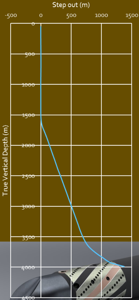
Vertical Section
