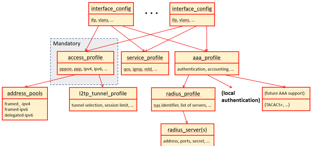
Figure 4. Access Profile Configuration and Overall Subscriber Management.
