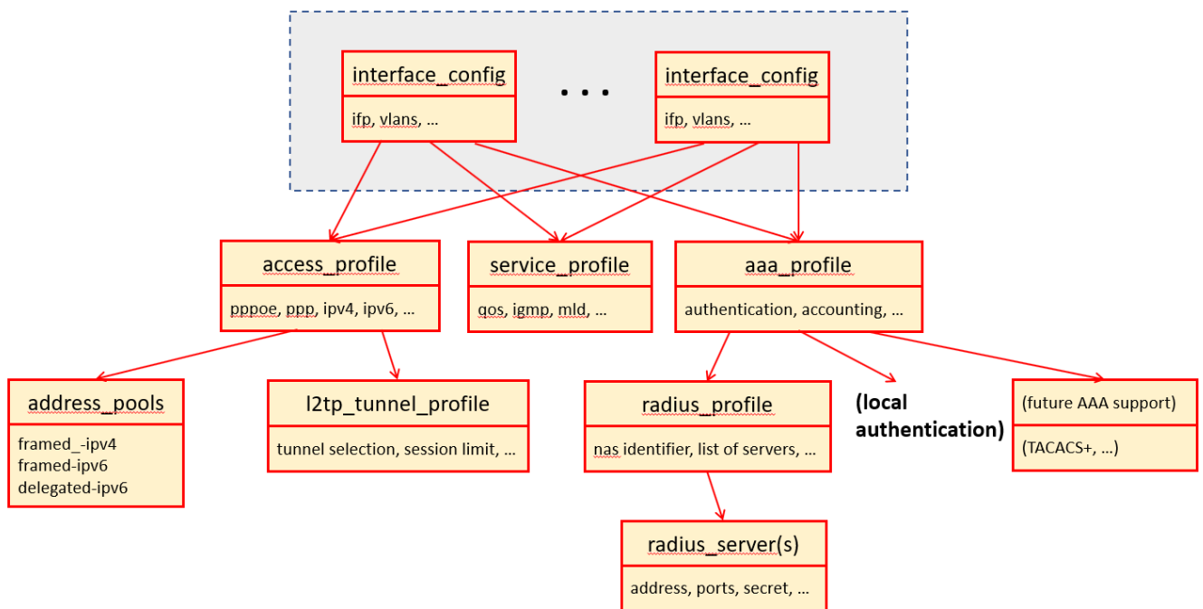
Figure 3. Access Interface Configuration and Overall Subscriber Management.
