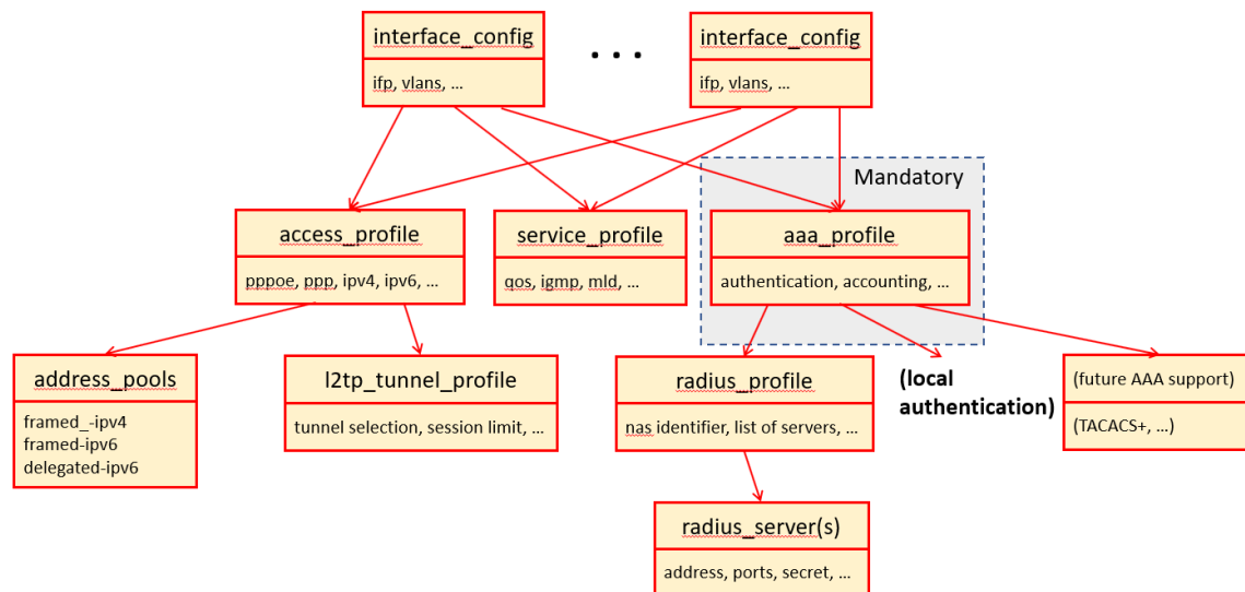
Figure 5. AAA Profile Configuration and Overall Subscriber Management.
