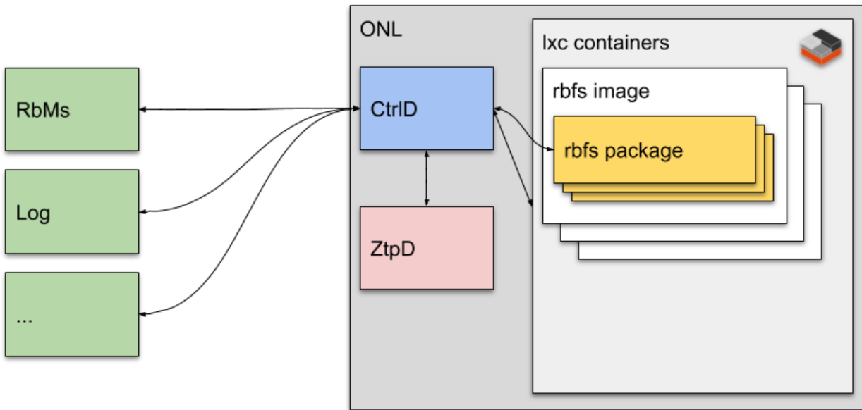
Figure 1: Overview of CTRLD.
