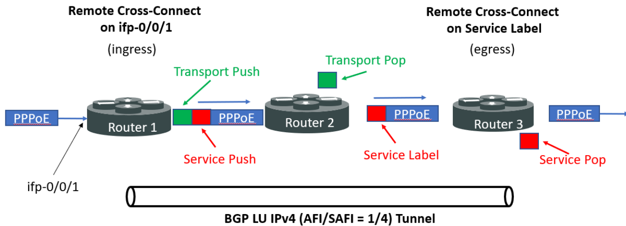
Figure 1. Remote Cross-Connect with MPLS tunnel.
